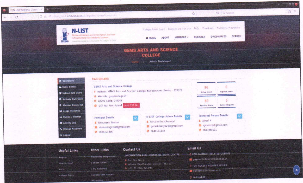
N-list -Dashboard
